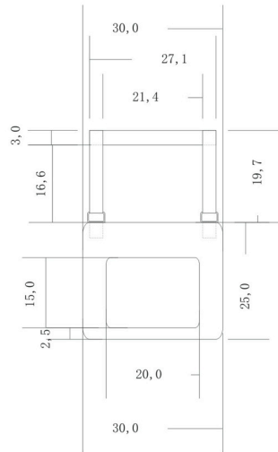
Vista Frontal
