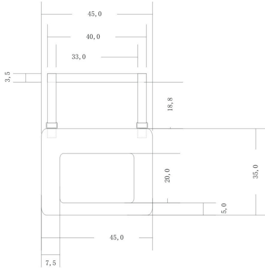
Vista Frontal
