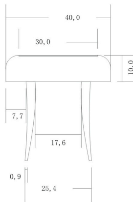
Vista Frontal
